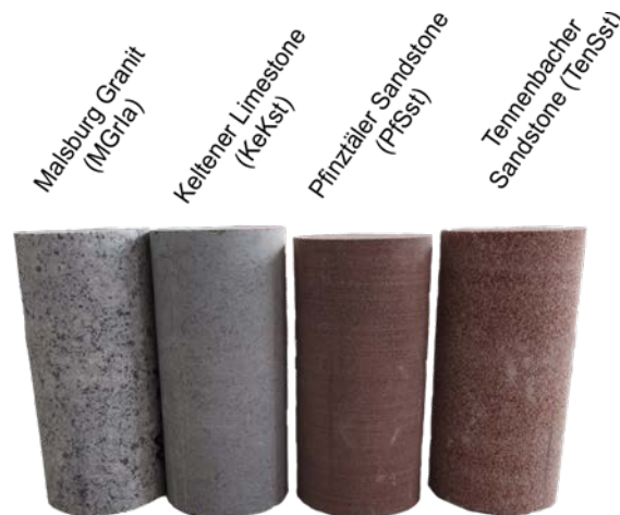
Figure 3: Figure of the four investigated rock samples. From left to right: The “Malsburg Granite” as a bright biotite granite with a homogeneous grain size distribution. The “Keltener Limestone”, a shell-bearing limestone alternated by fine grained parts. Fine grained “Pfinztaeler Sandstone” partly laminated with mica. Middle grained “Tennenbacher Sandstone”, a very homogeneous composed sandstone with high porosity.
